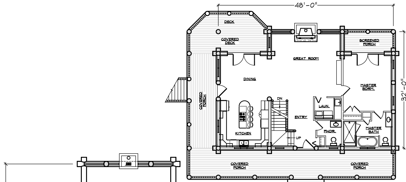
MAIN FLOOR PLAN
