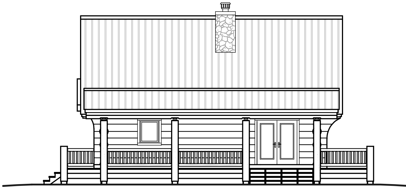
LEFT ELEVATION
