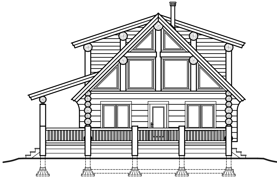
FRONT ELEVATION
