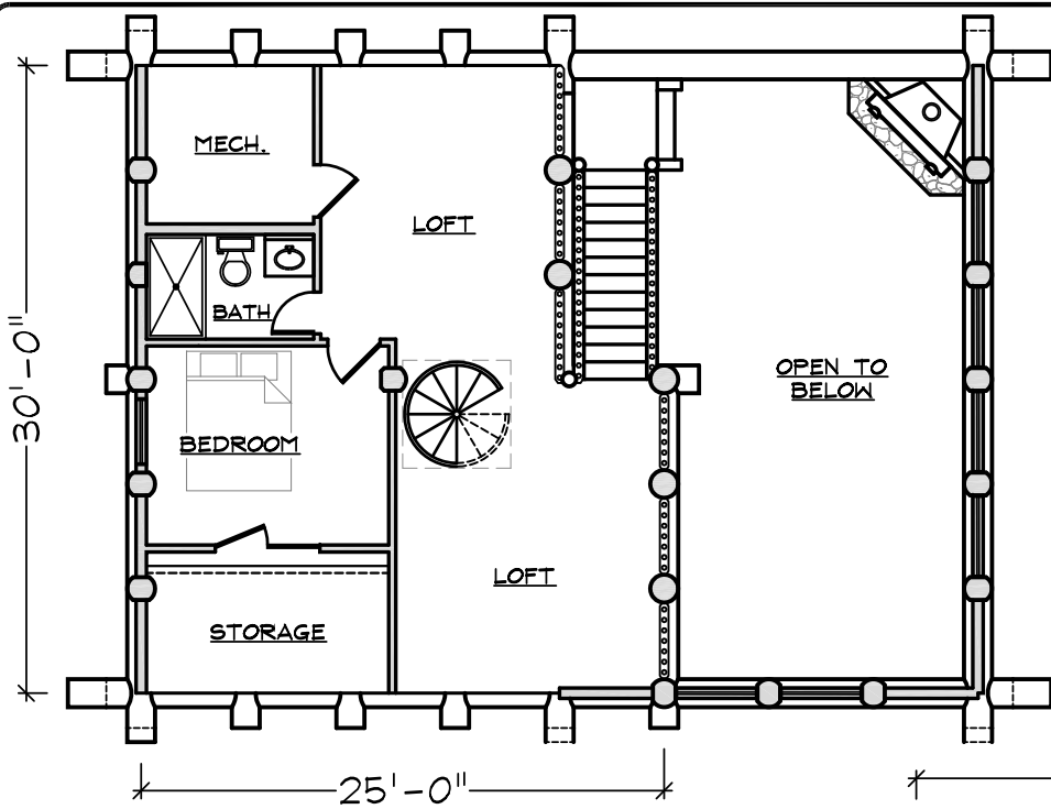
UPPER PLAN
