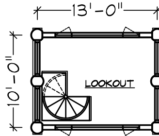
LOOKOUT PLAN
