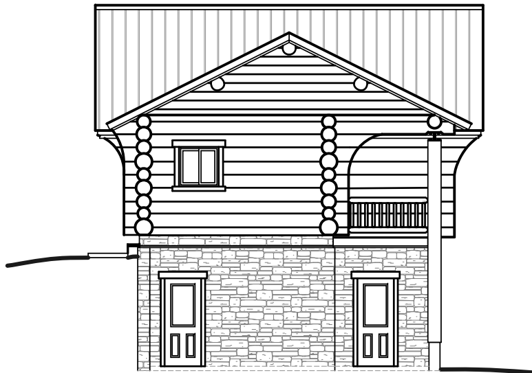
LEFT ELEVATION
