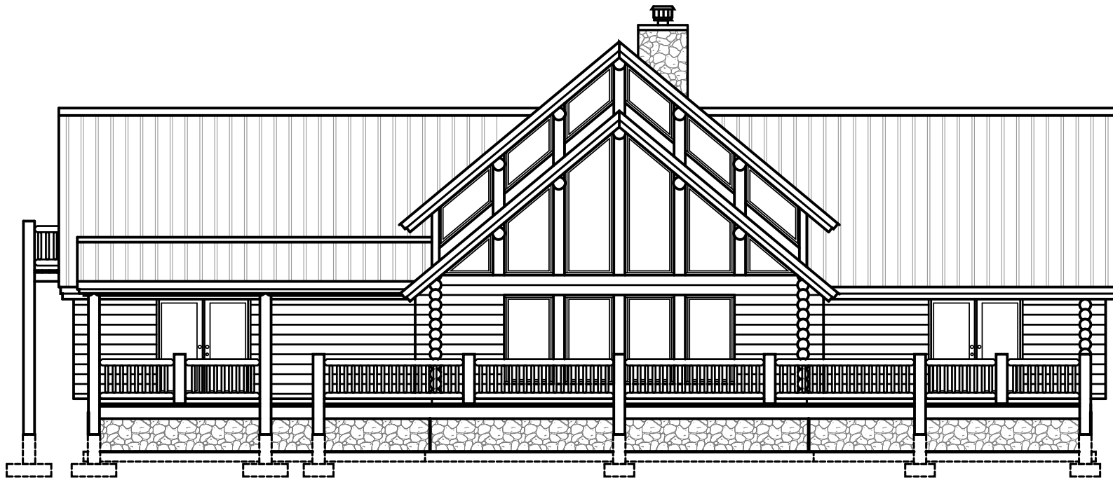
FRONT ELEVATION
