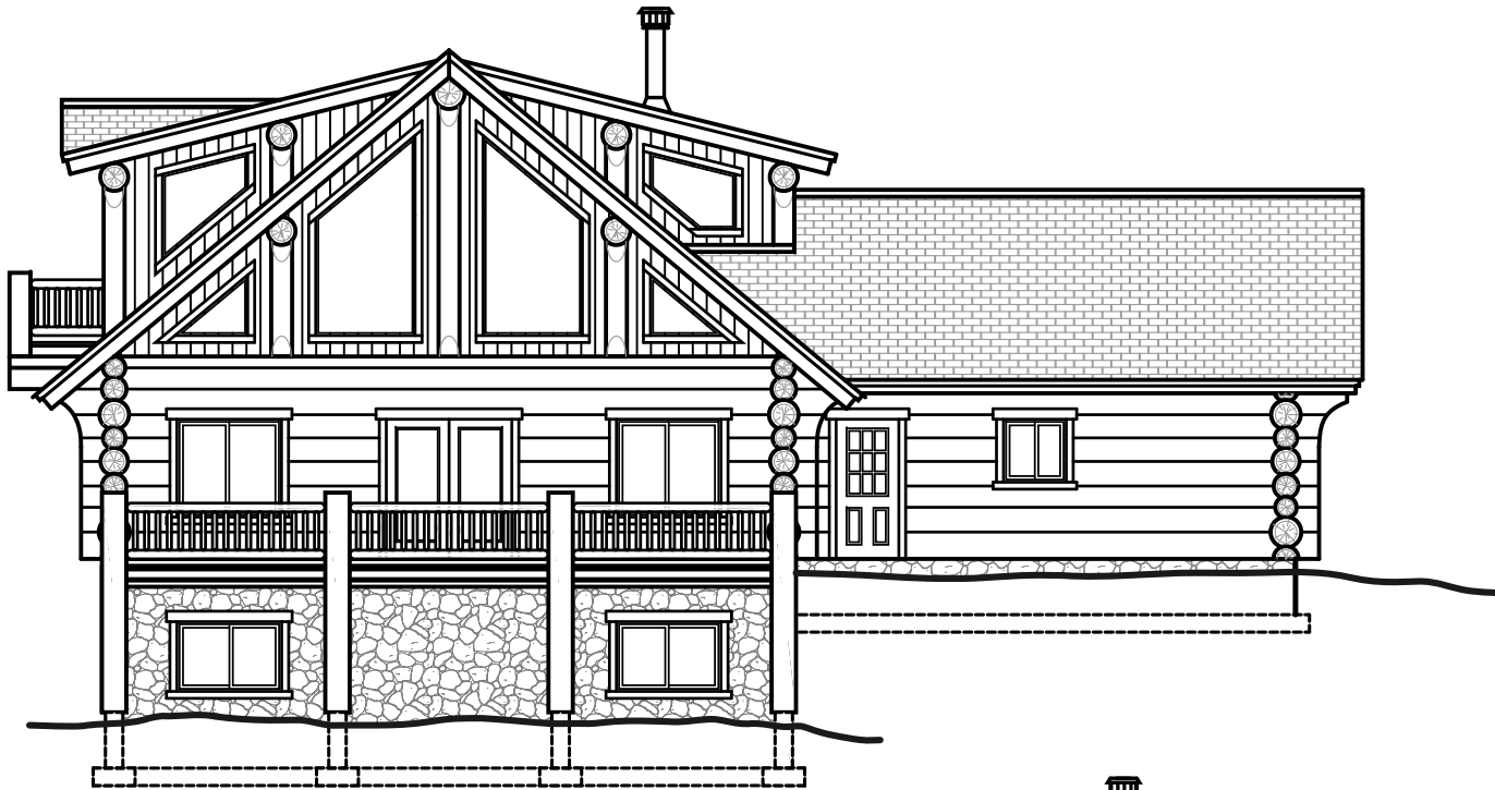
REAR ELEVATION
