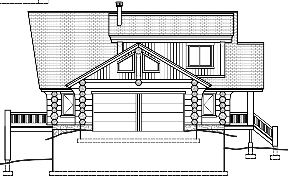
LEFT ELEVATION
