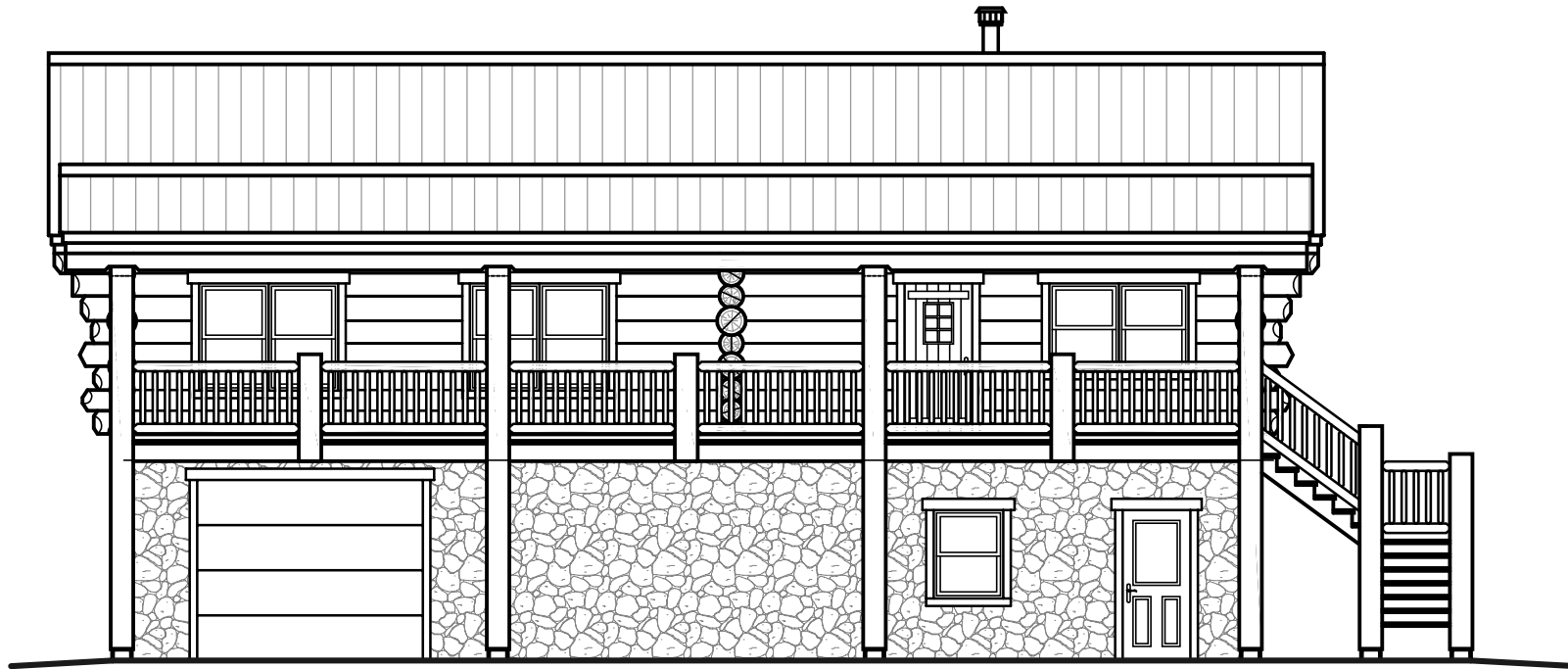
FRONT ELEVATION
