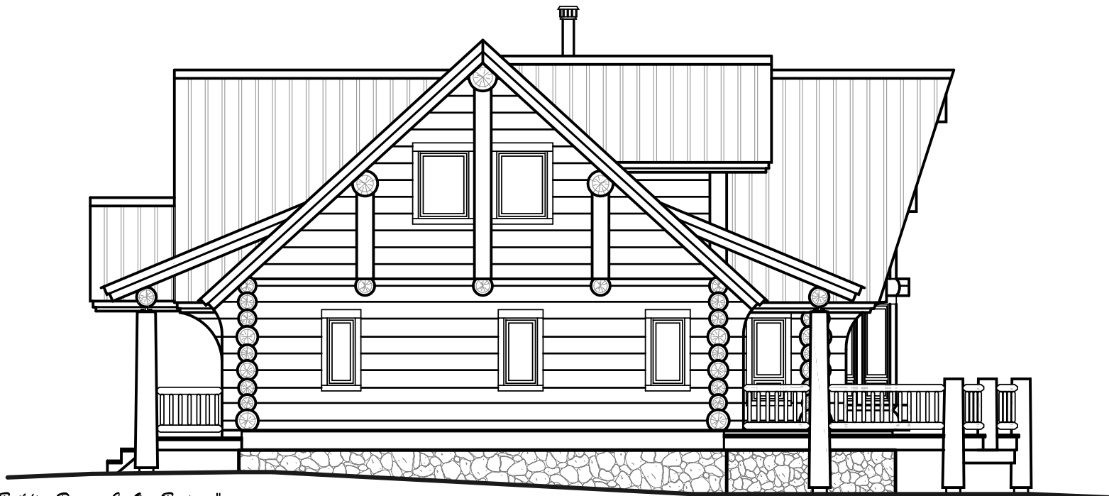
LEFT ELEVATION
