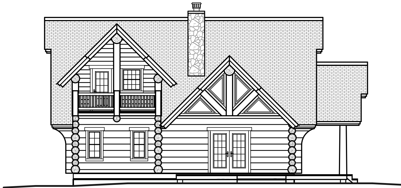
LEFT ELEVATION
